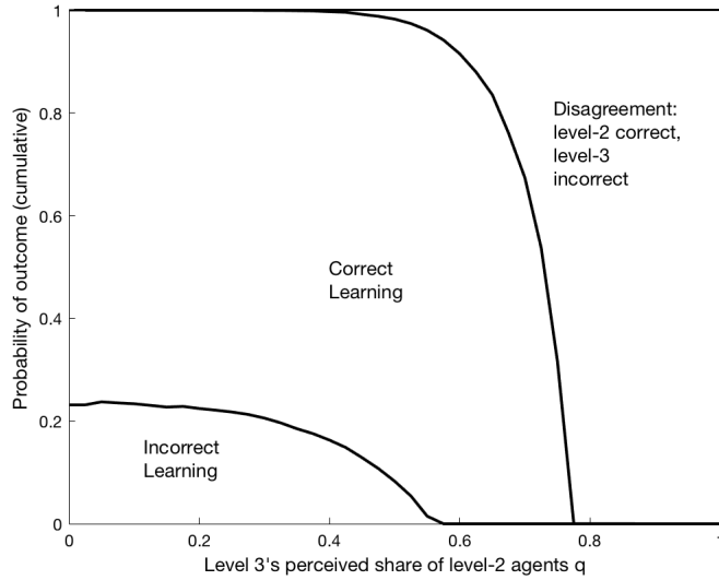
FIGURE F1. Cognitive Hierarchy Learning Outcomes (\omega = L, F^L(s) = \frac{10}{3}s - \frac{5}{3}s^2 - \frac{3}{5}, F^R(s) = \frac{5}{3}s^2 - \frac{1}{15})
