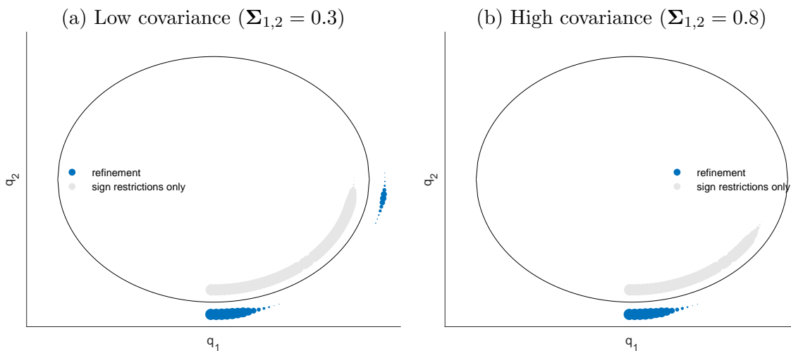
Figure 6: Simulated Identified Set for \mathbf{q} with Skew t Errors. Low vs High covariance. Truth near boundary.
