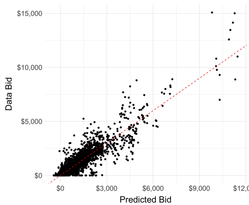
Figure 18: A scatter plot of actual quantities vs model predictions.
