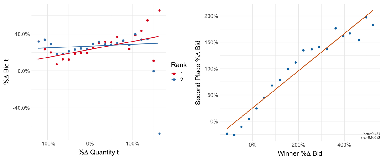
(a) Residualized bin-scatter of item-level percent overbid by the rank 1 (winning) and rank 2 bidder, against percent quantity overrun. (b) Bin-scatter of item-level percent overbids by the rank 2 bidder against the rank 1 (winning) bidder.
