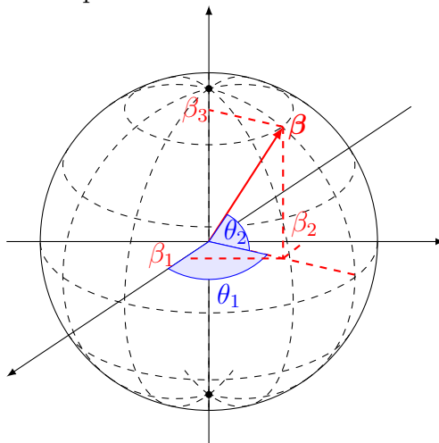
Figure 2: Reparameterization of the Unit Sphere
