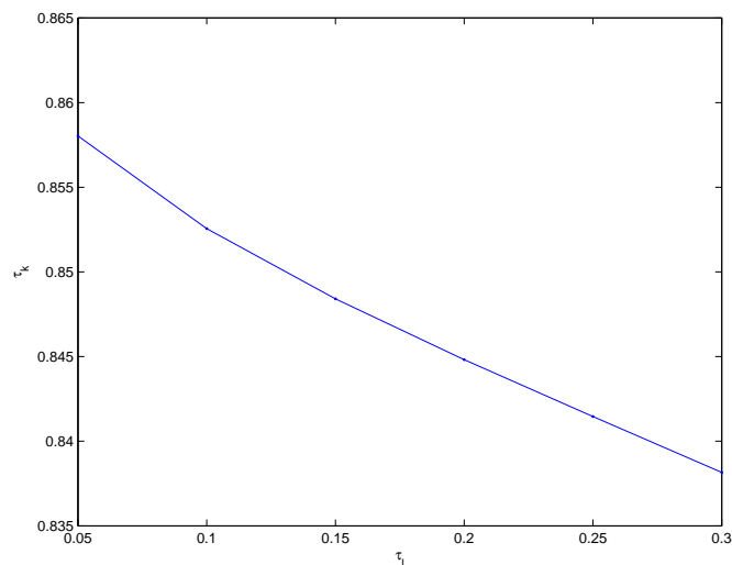
Figure 2: \tau_k , optimal s.s. capital tax
