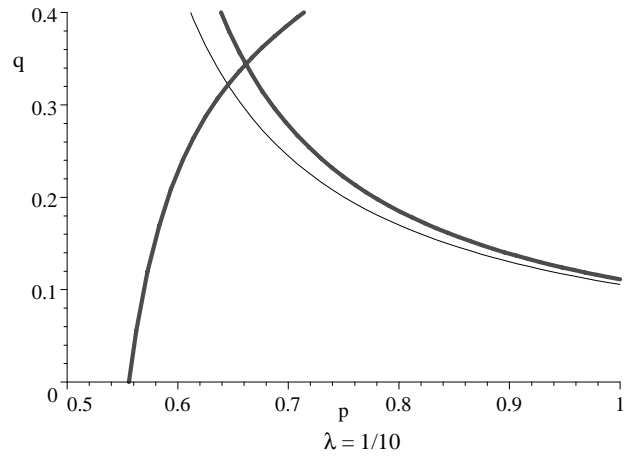
Figure 5: Bias-driven debate equilibrium (\hat{p}, \hat{v})
