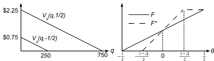
Figure 2: Inverse demand curves and priors in example 1.
