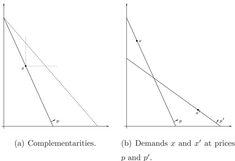
FIGURE 1. When is observed demand consistent with complementarity?
