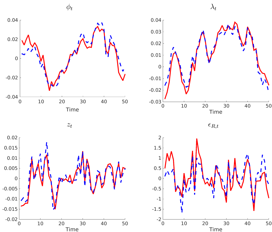
Figure 25: Particle-Filtered States
