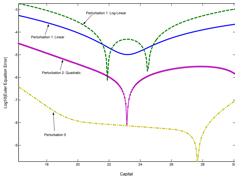
Figure 14: \log_{10} of Absolute Value of Euler Equation Error
