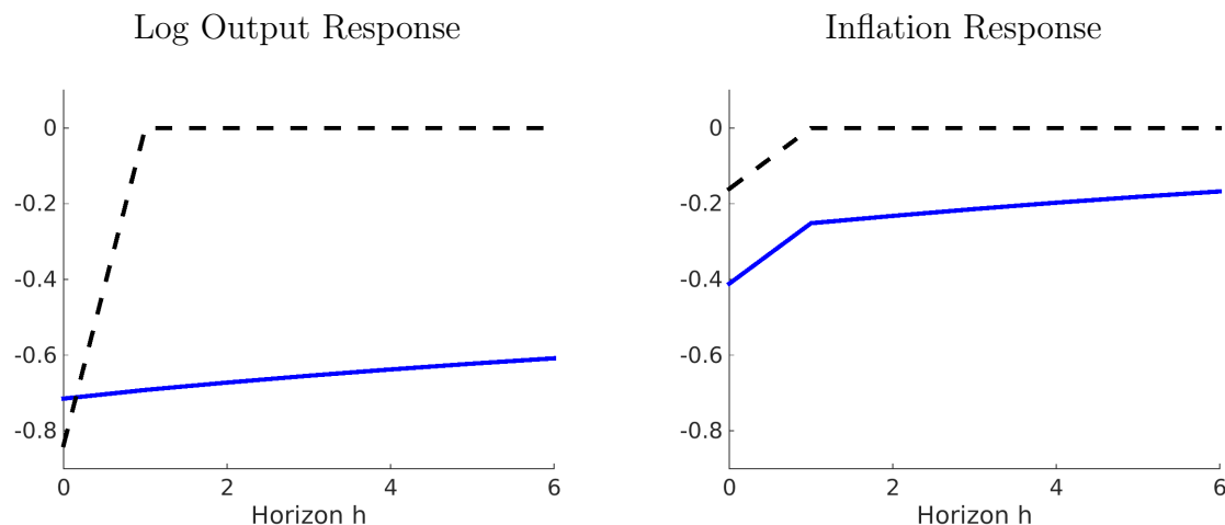
Figure 29: DSGE Model and VAR Impulse Responses to a Monetary Policy Shock
