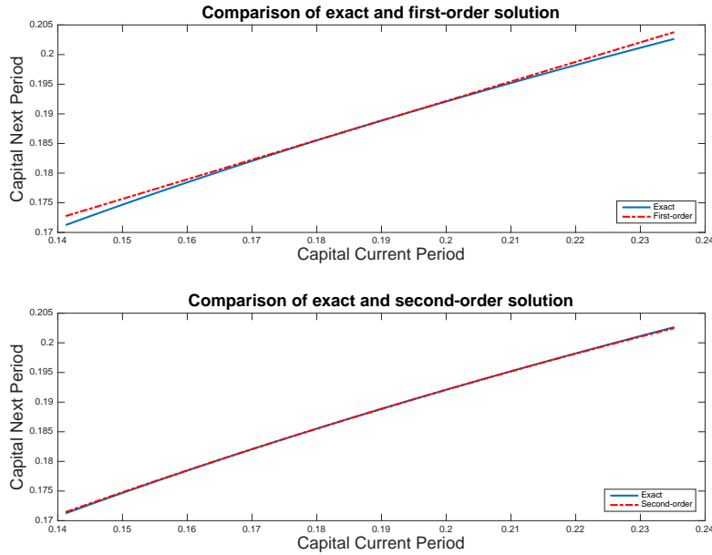
Figure 1: Comparison of Exact and Perturbation Solution
