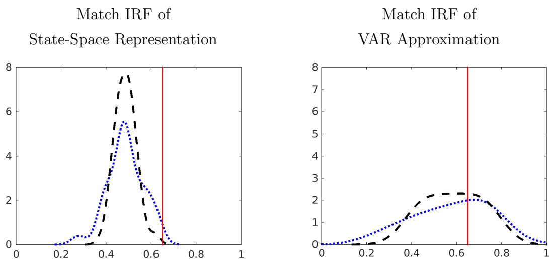
Figure 31: Sampling Distribution of \hat{\zeta}_{p,irf}
