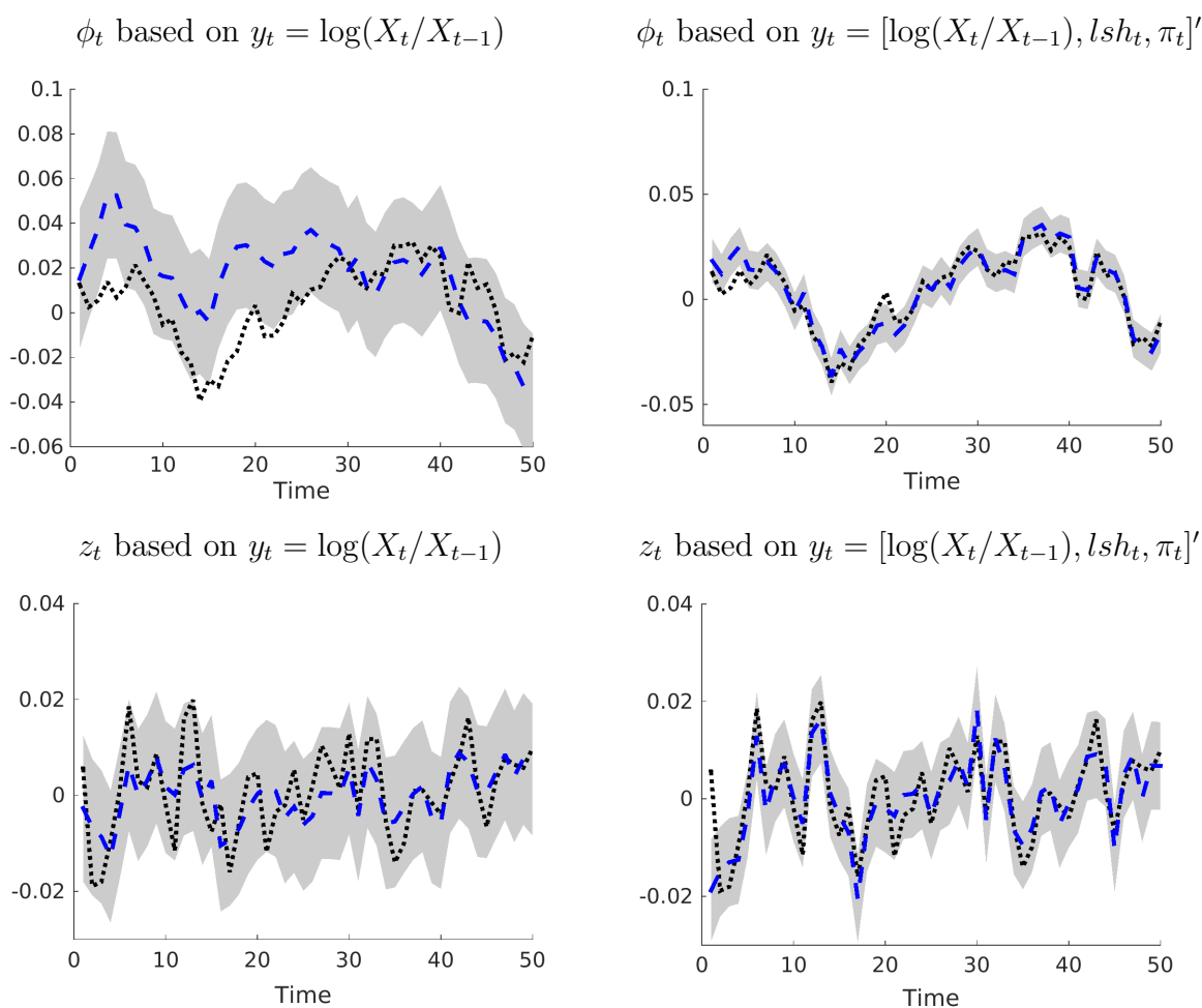
Figure 24: Filtered States
