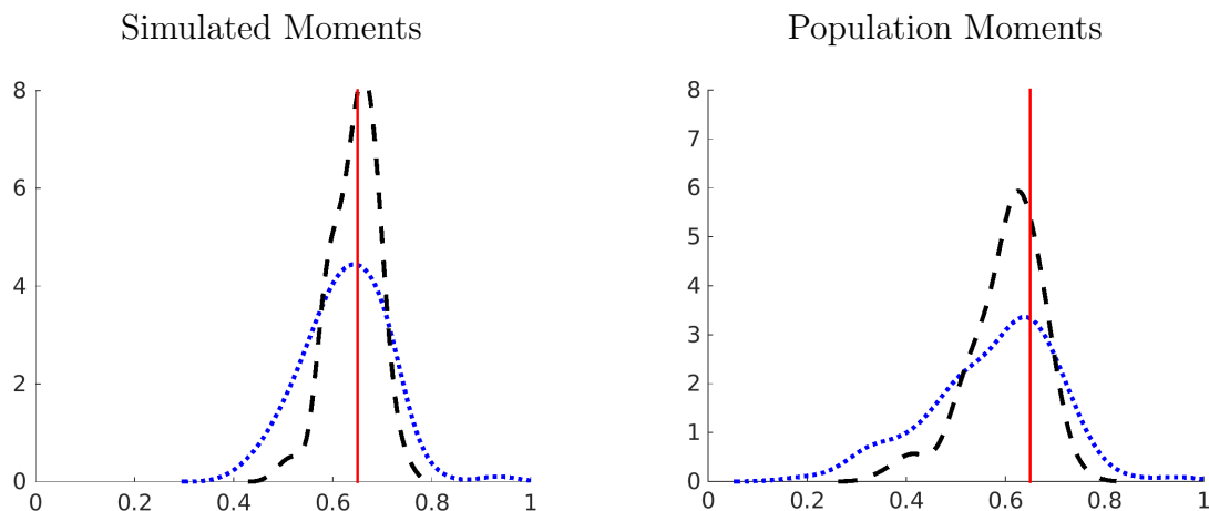
Figure 28: Sampling Distribution of \hat{\zeta}_{p,md}
