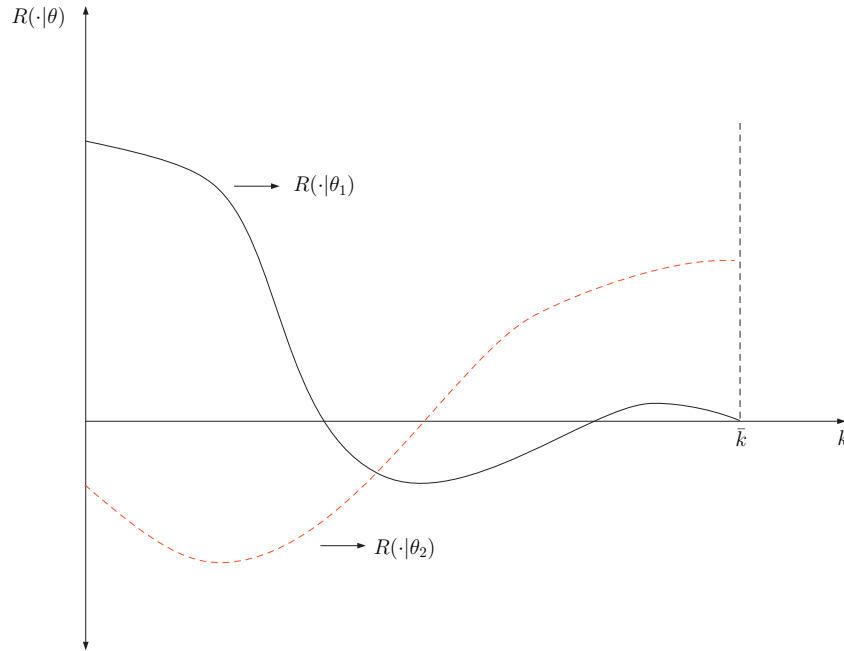
Figure 2: Residual Functions
