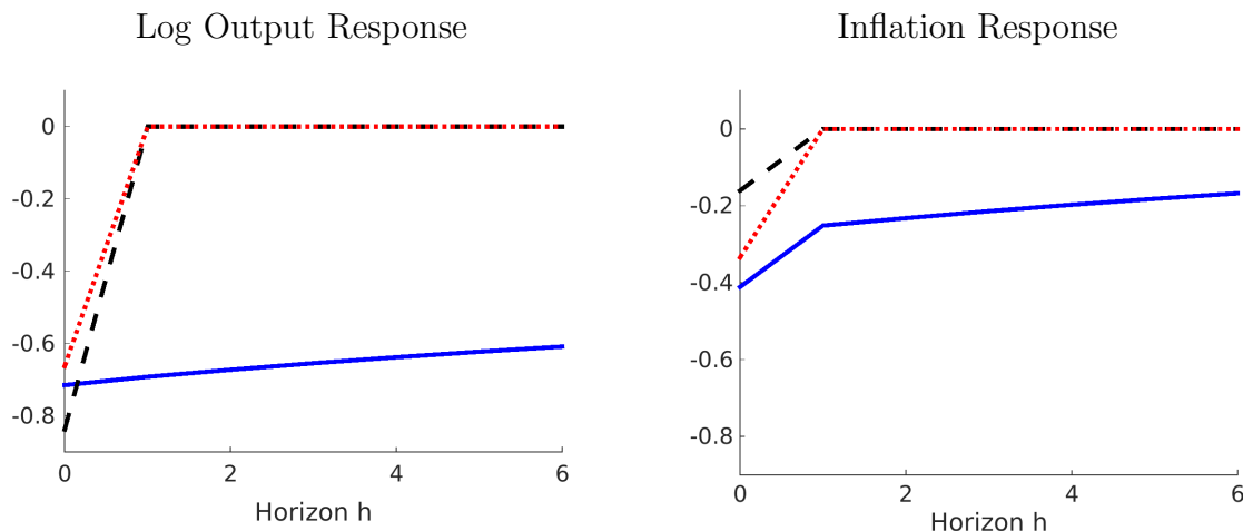
Figure 30: Sensitivity of IRF to \zeta_p
