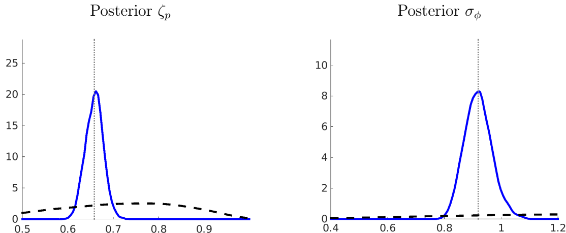
Figure 33: Prior and Posterior Densities
