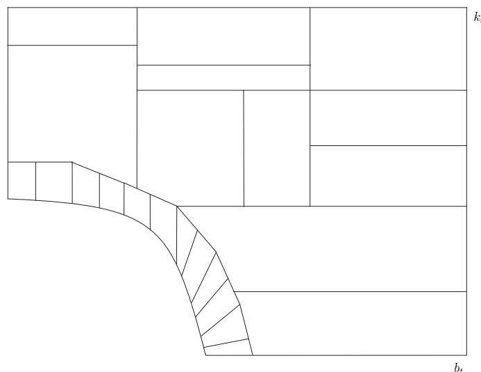
Figure 7: 2-Dimensional Element Grid
