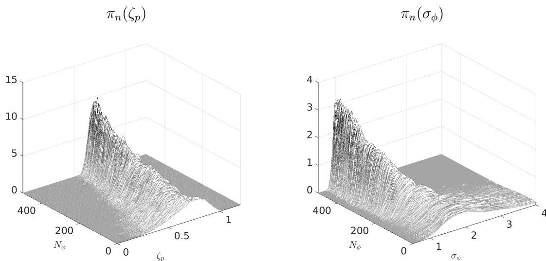
Figure 34: SMC Bridge Densities
