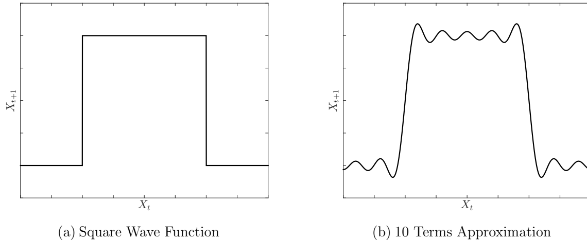
Figure 4: Gibbs Phenomenon
