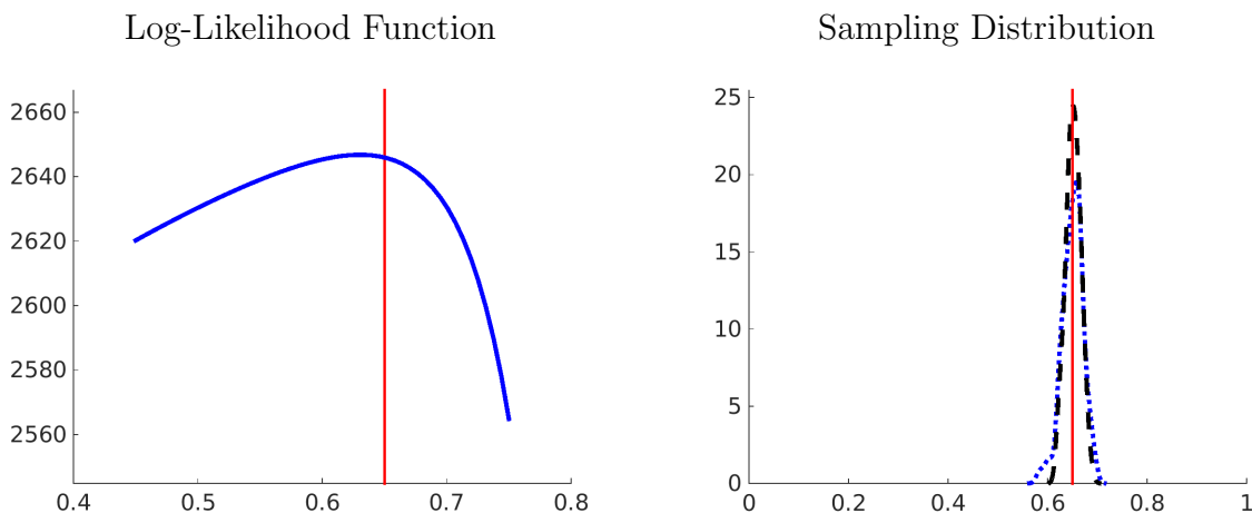
Figure 27: Log-Likelihood Function and Sampling Distribution of \hat{\zeta}_{p,ml}
