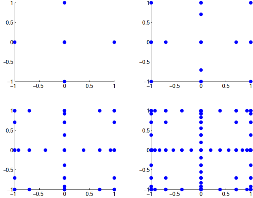
Figure 11: Four Sparse Grids
