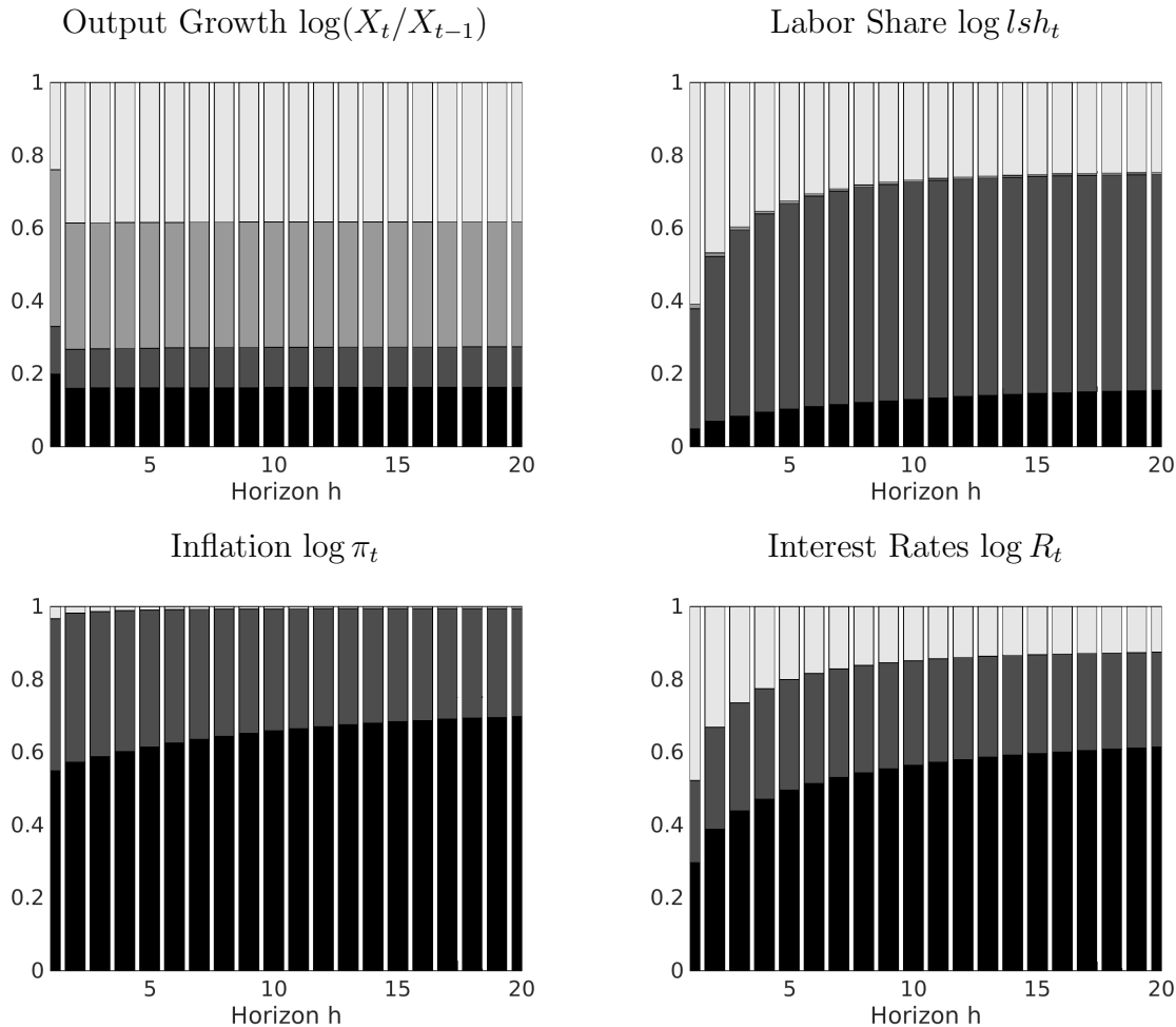
Figure 17: Forecast Error Variance Decomposition
