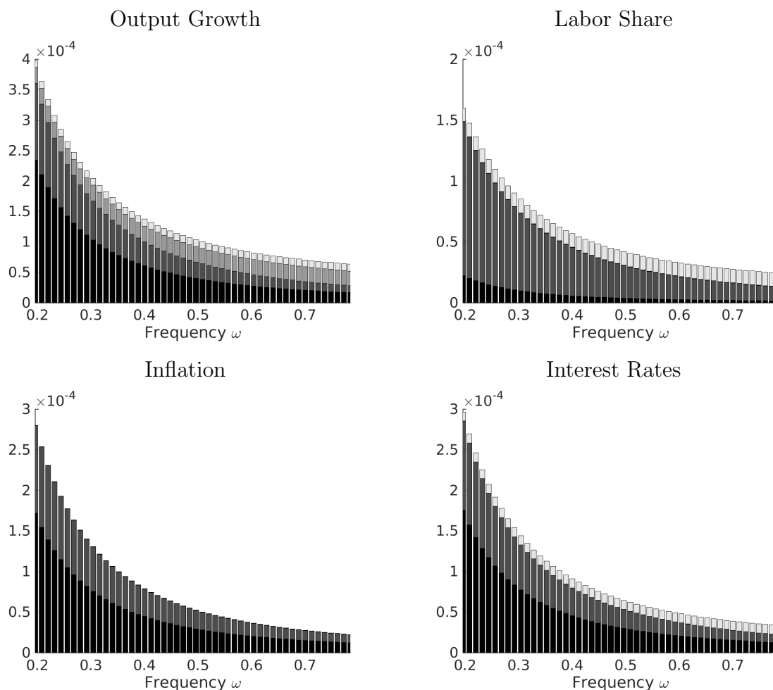
Figure 18: Spectral Decomposition
