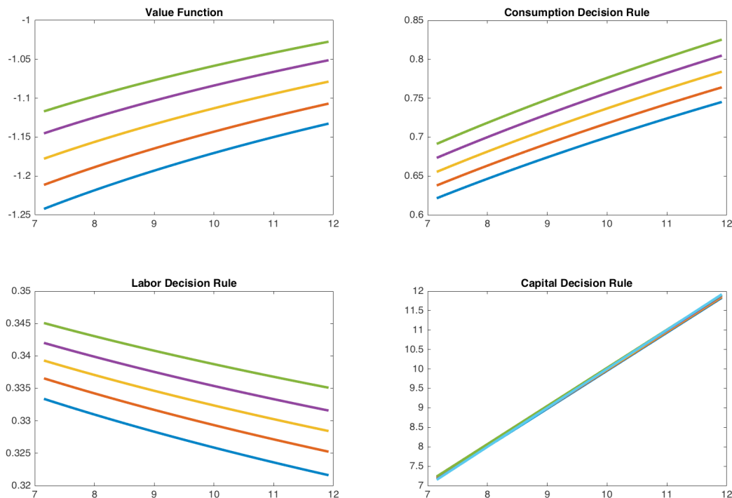
Figure 10: Solution, Stochastic Neoclassical Growth Model
