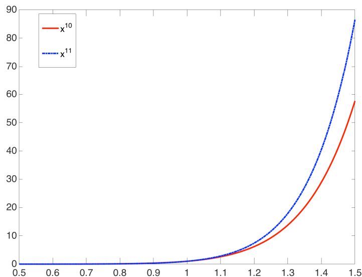
Figure 5: Graphs of x^{10} and x^{11}
