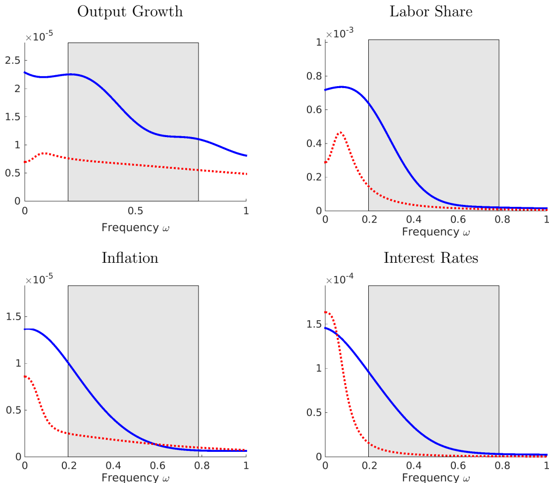
Figure 21: Empirical Spectrum
