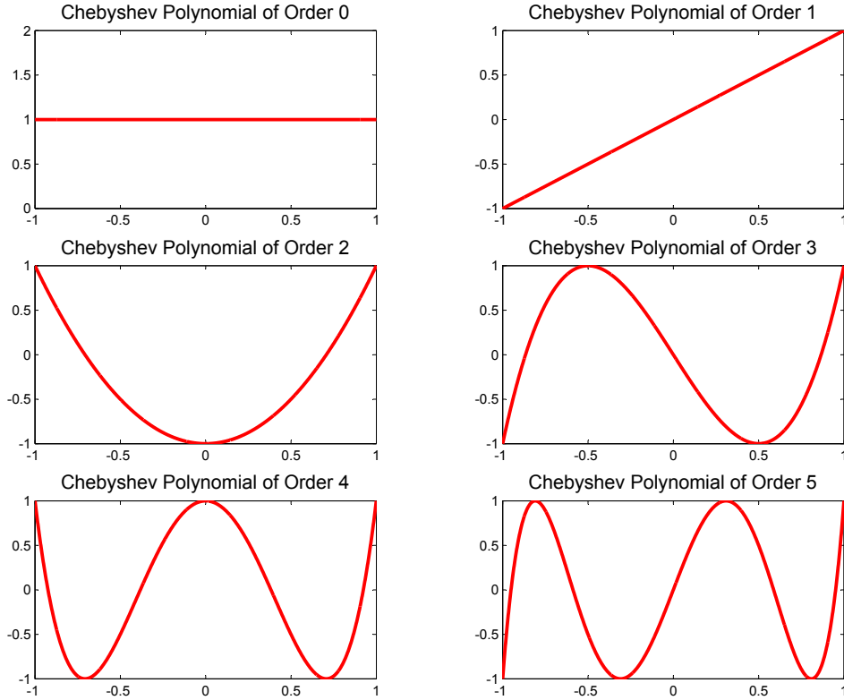
Figure 6: First Six Chebyshev Polynomials
