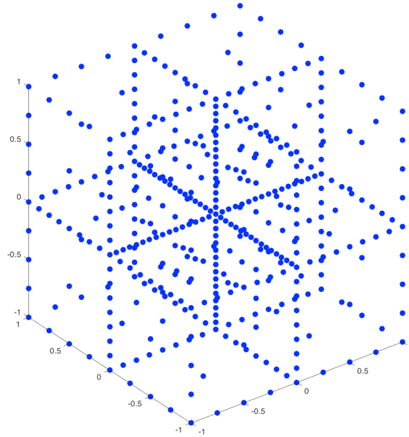
Figure 12: A Sparse Grid, 3 State Variables
