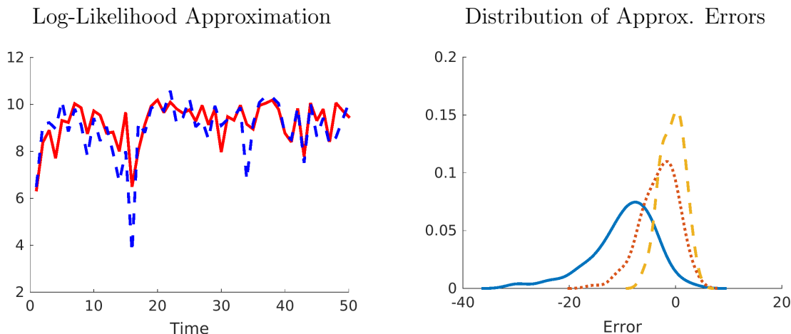
Figure 26: Particle-Filtered Log-Likelihood
