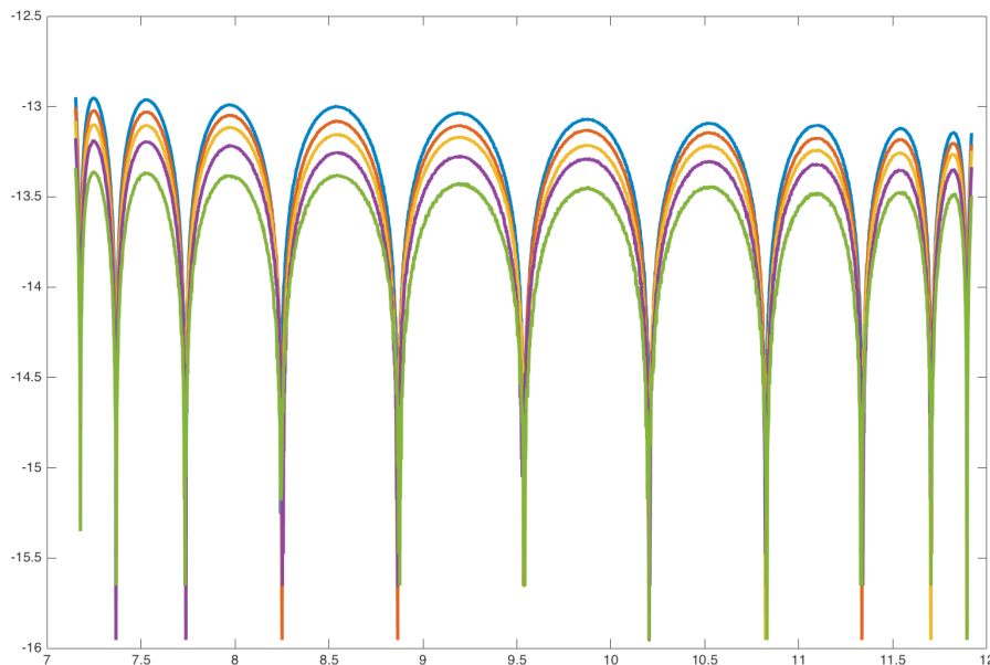
Figure 13: \log_{10} of Absolute Value of Euler Equation Error
