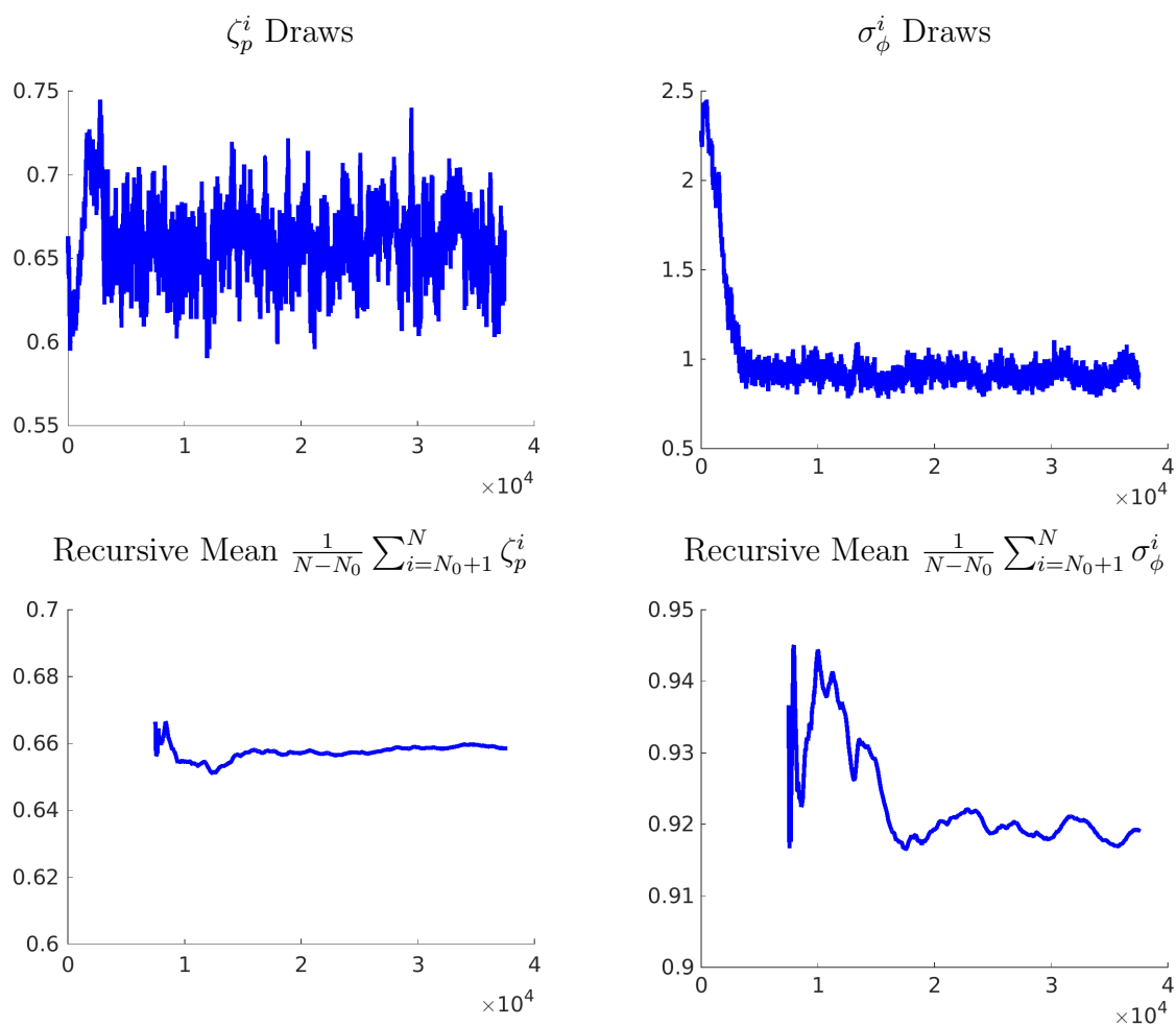
Figure 32: Parameter Draws from MH Algorithm
