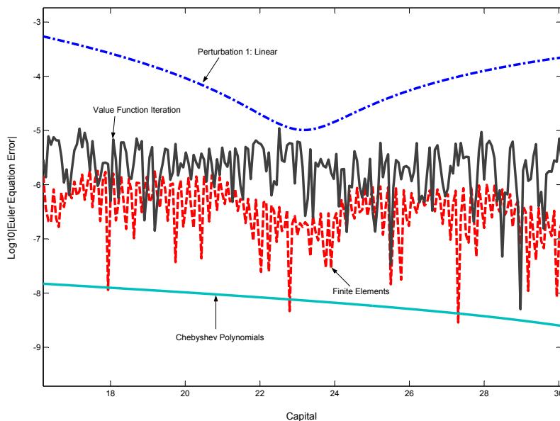
Figure 15: \log_{10} of Absolute Value of Euler Equation Error
