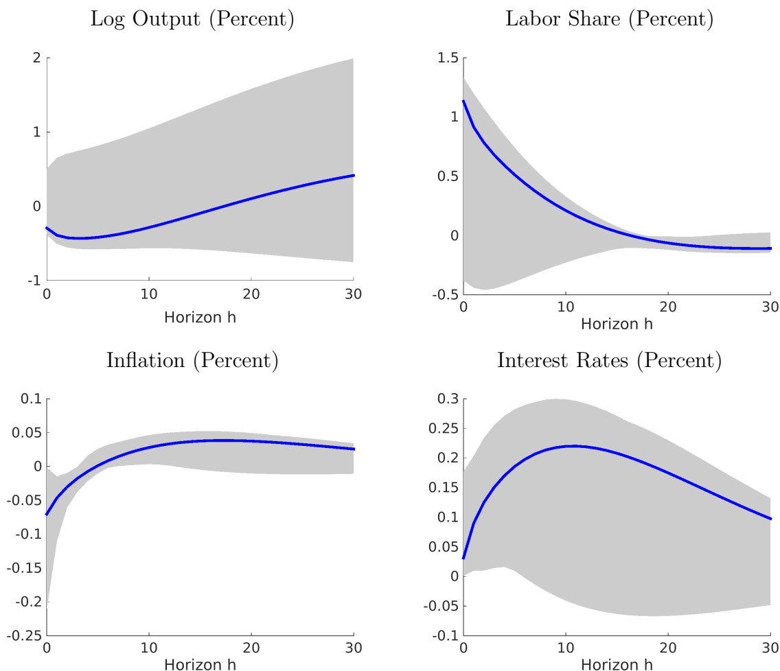
Figure 22: Impulse Responses to a Monetary Policy Shock
