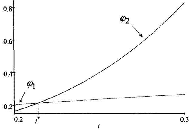
Figure 5: The net surplus functions corresponding to bs and 2(bs)^2 , where \varphi_1(i) = \max_{b,s} bs - \psi(b, i) - c(s, i) and \varphi_2(i) = \max_{b,s} 2(bs)^2 - \psi(b, i) - c(s, i) .
